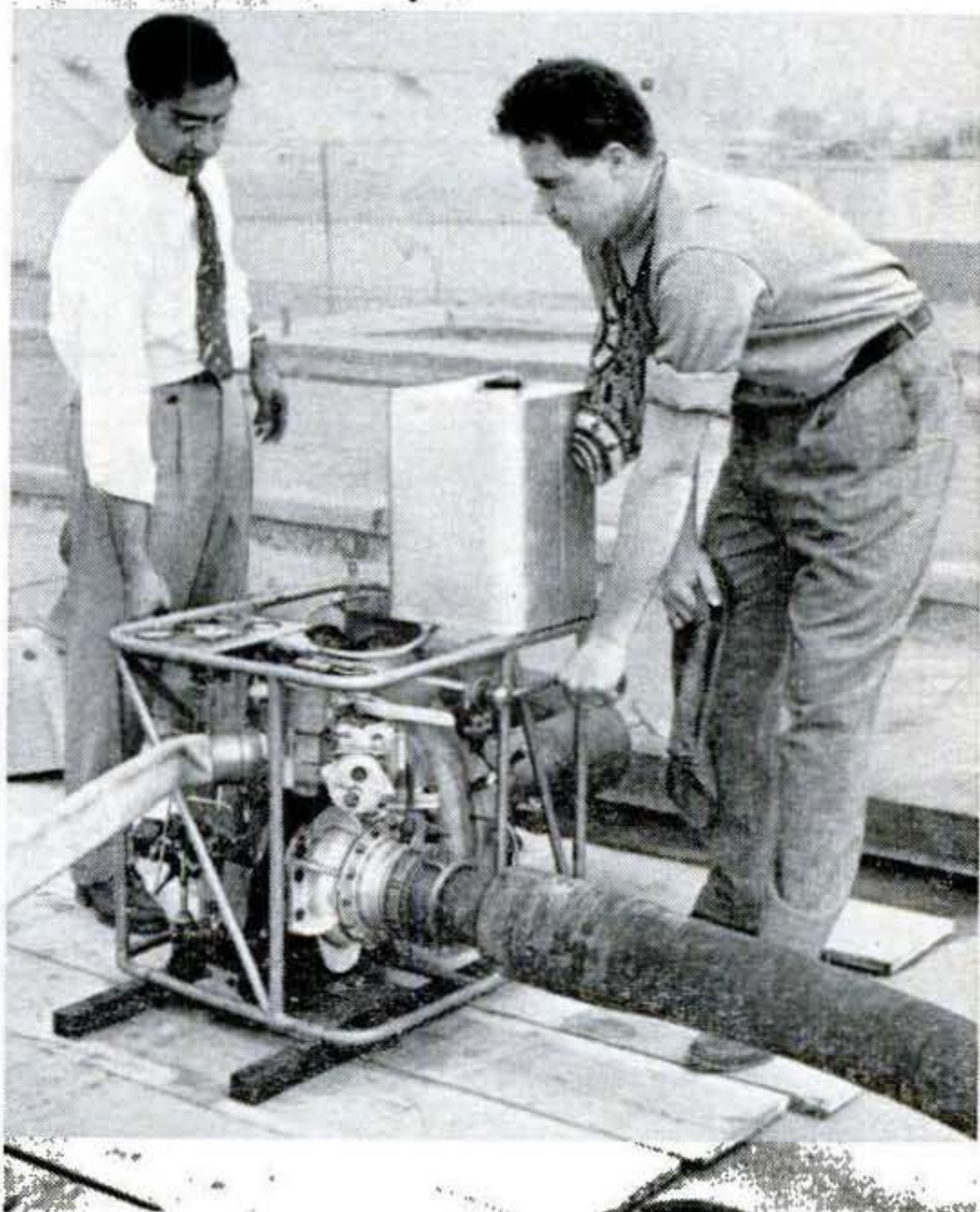
TWO HAND CRANKS spin turbine at 11,000 to 12,000 r.p.m. Then its own power takes over. It has two seven-gallon fuel tanks, one of which is shown installed above.
